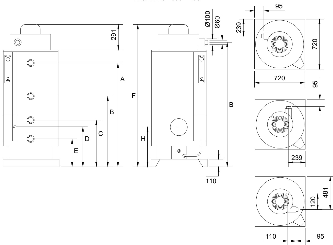
fig. 1.6/3 misure in mm
