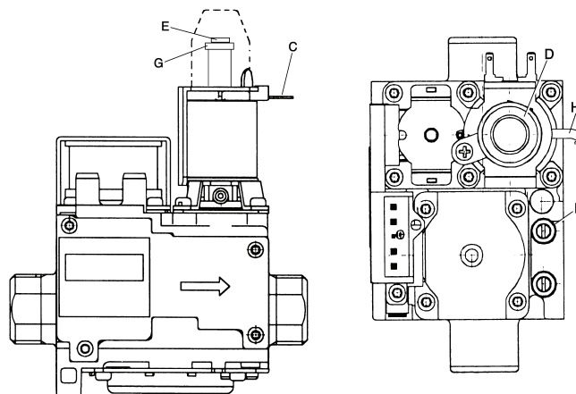
fig. 22 - Valvola gas
