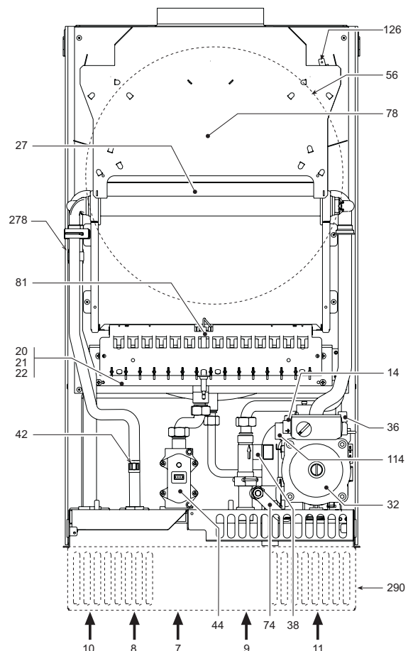
fig. 14 - Vista general TAURA D 32 MCA
