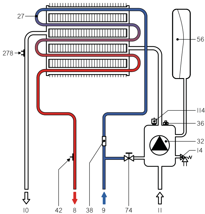
fig. 16 - Circuito de AS
